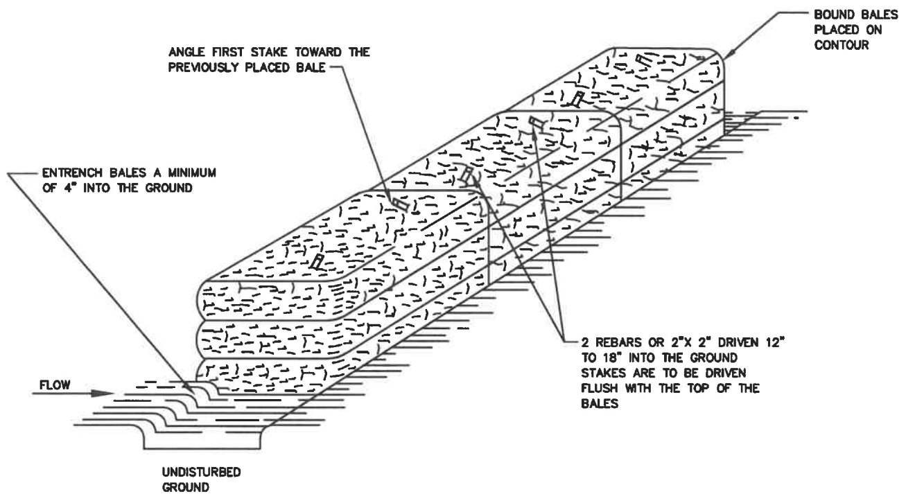
ANCHORING DETAIL
