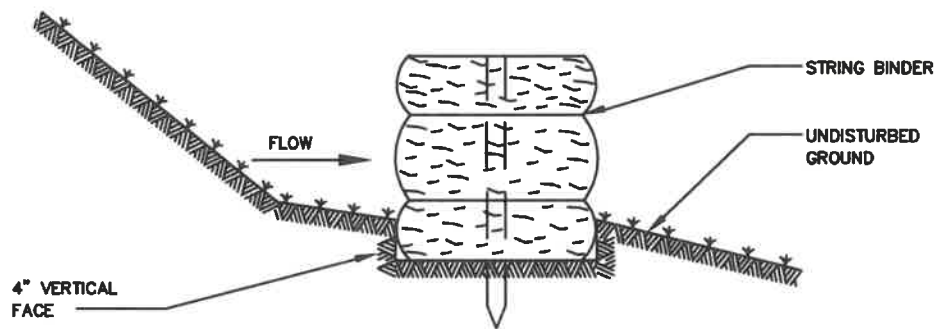
BEDDING DETAIL
