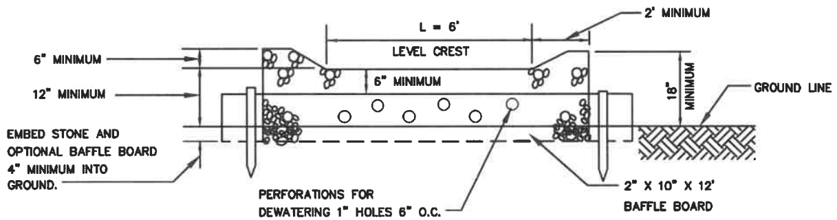
CROSS SECTION
